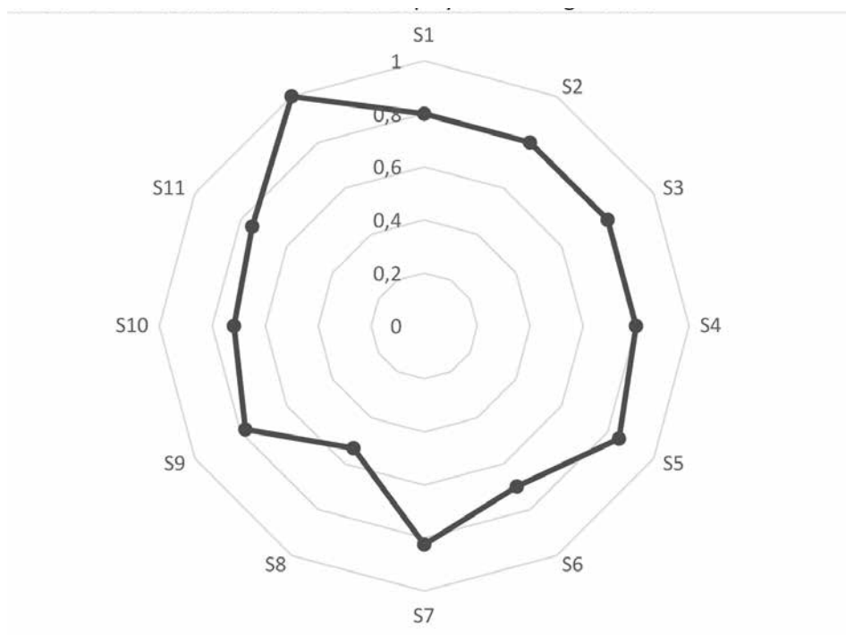
Figure 4: Spearman's coefficient values for ranking changes correlation between criteria coefficients
